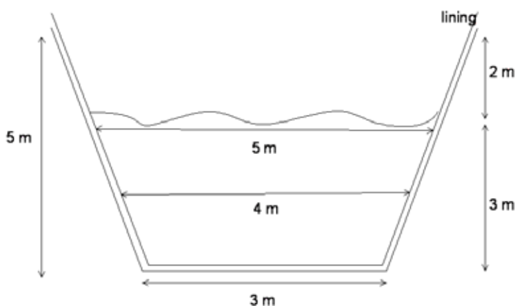
Figure A6.2 Example of the dimensions of a battered burial pit
